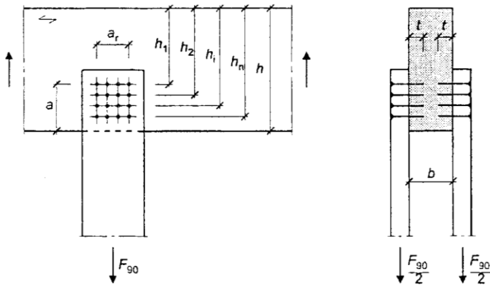
Figure 1: Example of connection with nails.
