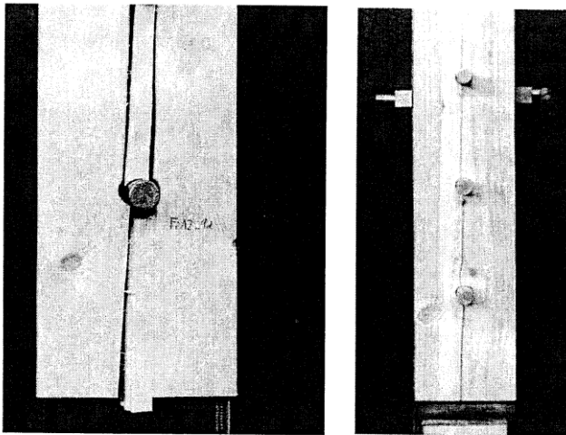
Fig. 1: plug shear failure
