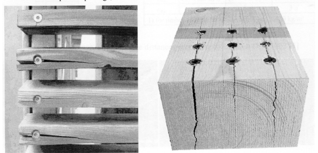
Fig. 1: Typical splitting failure caused by the insertion of self-tapping screws
