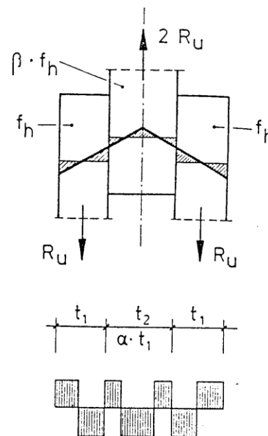
b)static model of the failure mode
