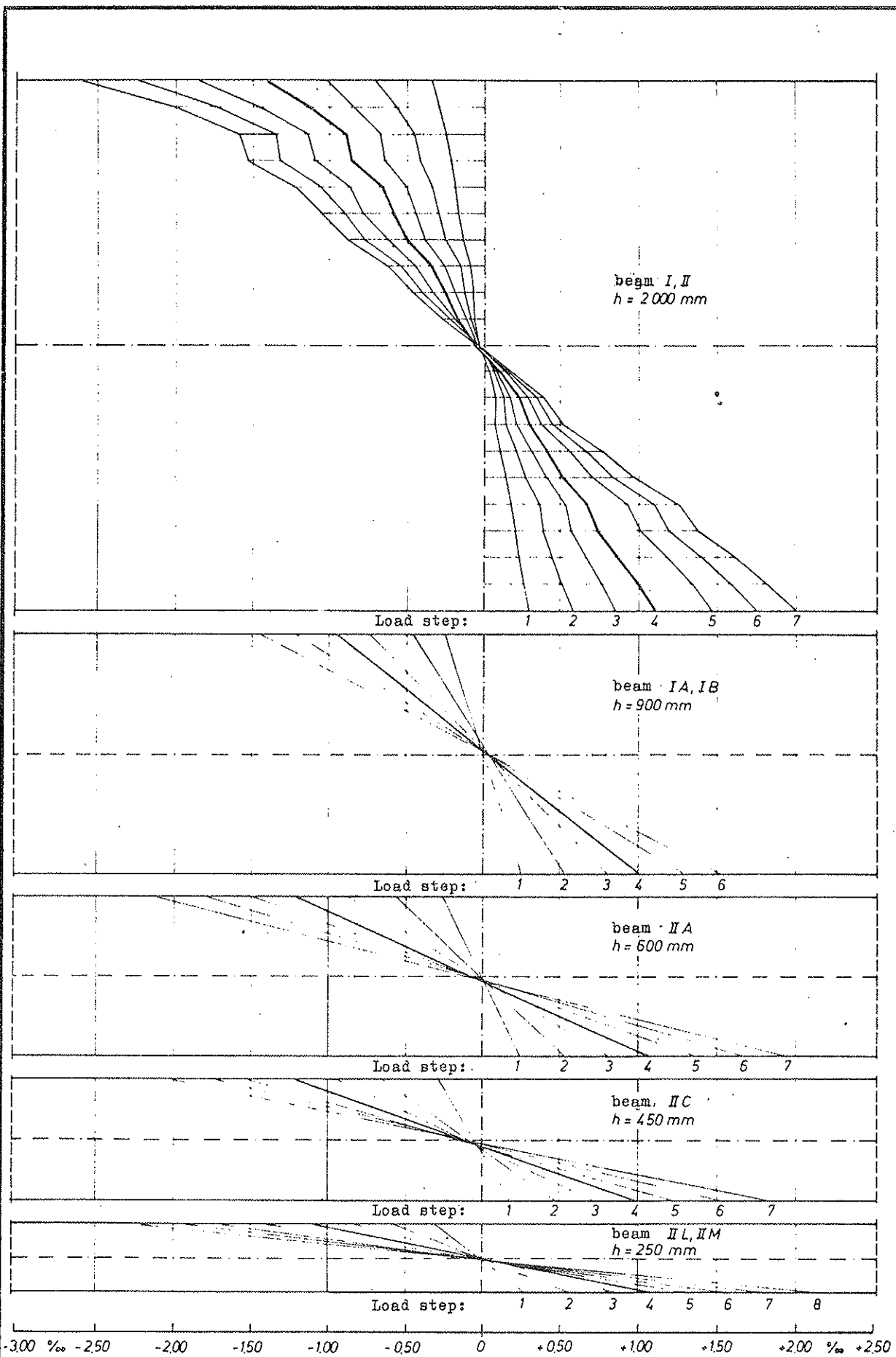
Fig. 2 Longitudinal stresses at different beam depths
